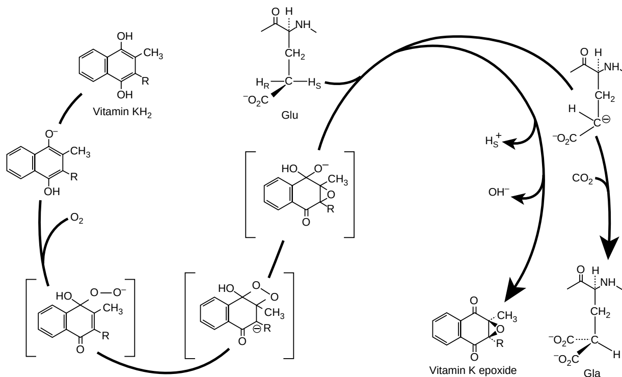
FIGURE 2 The vitamin K-dependent, \gamma -glutamyl carboxylase. The available data support an interaction of \text{O}_2 with vitamin \text{KH}_2 , the reduced (hydronaphthoquinone) form of vitamin K, to form an oxygenated intermediate which is sufficiently basic to abstract the \gamma -hydrogen of the glutamyl residue. The products of this reaction are vitamin K-2,3-epoxide and a glutamyl carbanion. Attack of \text{CO}_2 on the carbanion leads to the formation of a Gla residue. The bracketed peroxy, dioxetane, and alkoxide intermediates have not been identified in the enzyme catalyzed reaction but are postulated based on model organic reactions, and the available data are consistent with their presence.
