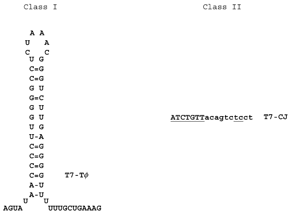
FIGURE 5 (Left) RNA structure of the T7 RNA polymerase T\phi class I terminator. Termination occurs at the underlined nucleotide. (Right) Nontemplate strand DNA sequence of the class II T7 RNA polymerase concatemer junction terminator.
